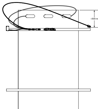
Illustration 2: Montage vertical
