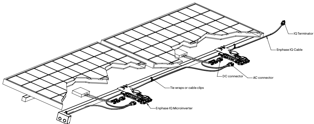
Illustration 1: Montage horizontal
