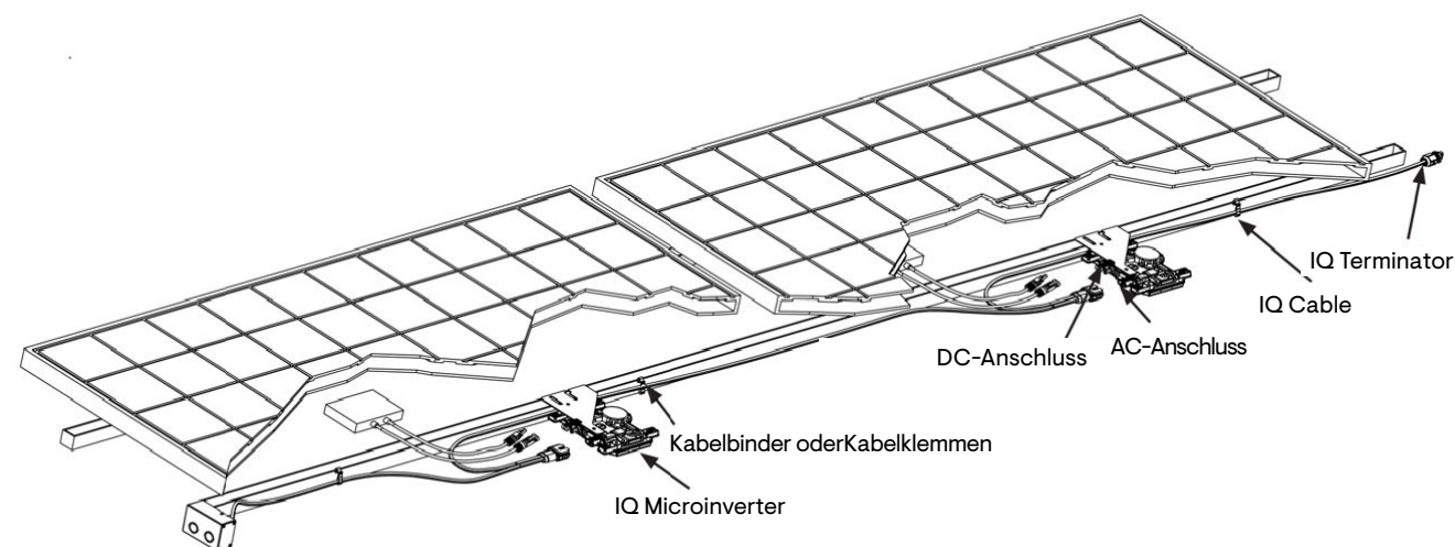
Illustration 1: Montage horizontal
