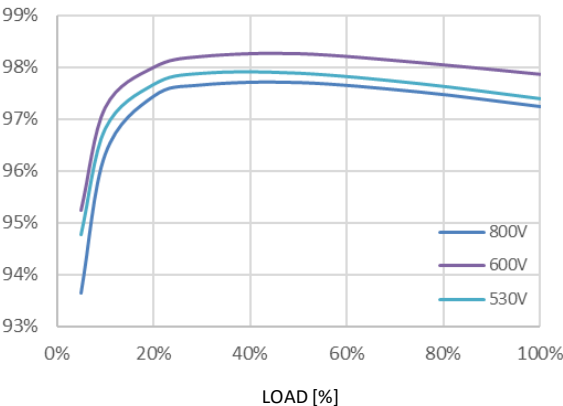
Efficiency Curve
