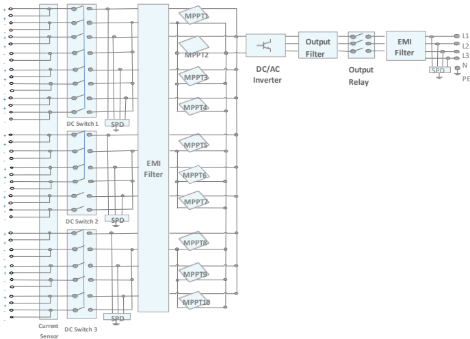
Circuit Diagram
