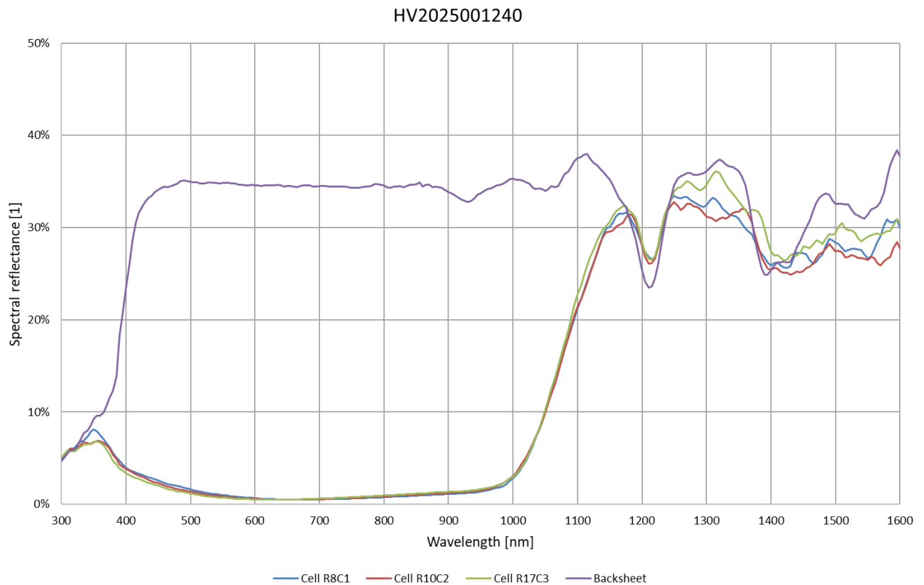
Measured spectral hemispherical reflectance curves (detail)
