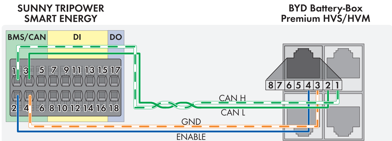
Figure 2: Cabling plan according to the TIA-568A standard: Sunny Tripower Smart Energy with BYD Battery-Box Premium HVM/HVS. The individual cable ends must be provided with a 12 mm long wire end sleeve.
